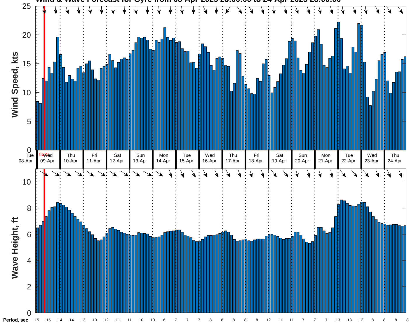
Wind & Wave Forecast for Gyre from 08-Apr-2025 23:00:00 to 24-Apr-2025 23:00:00
