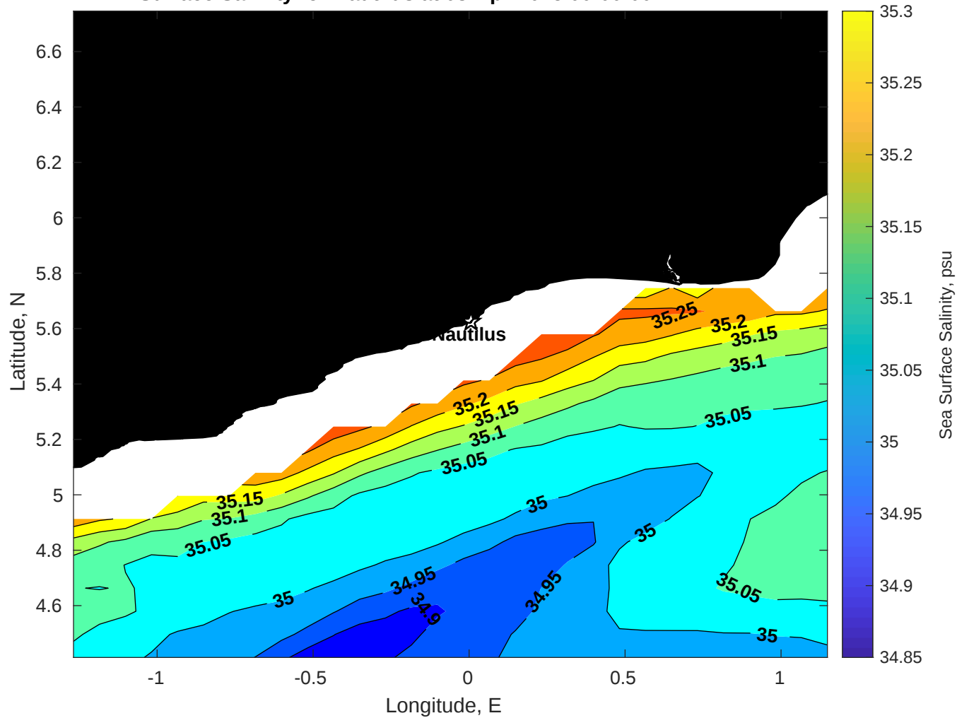
Surface Salinity for Nautilus at 08-Apr-2025 00:00:00
