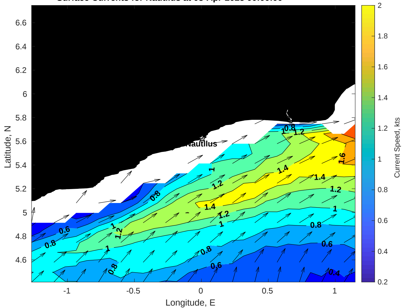
Surface Currents for Nautilus at 08-Apr-2025 00:00:00
