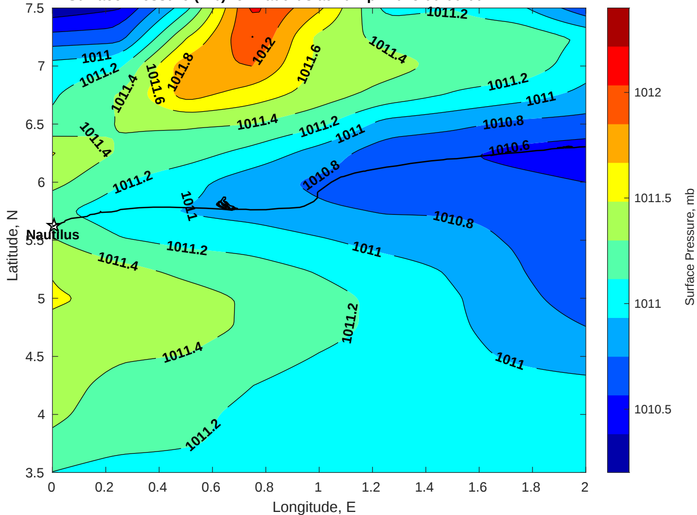
Surface Pressure (mb) for Nautilus at 10-Apr-2025 00:00:00
