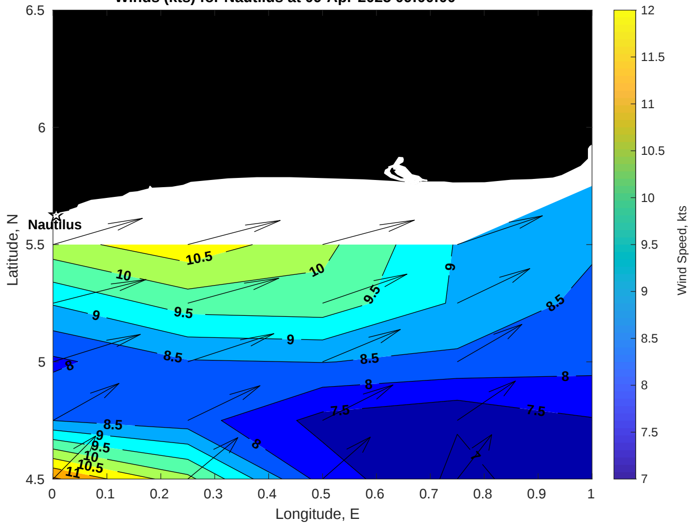
Winds (kts) for Nautilus at 09-Apr-2025 09:00:00
