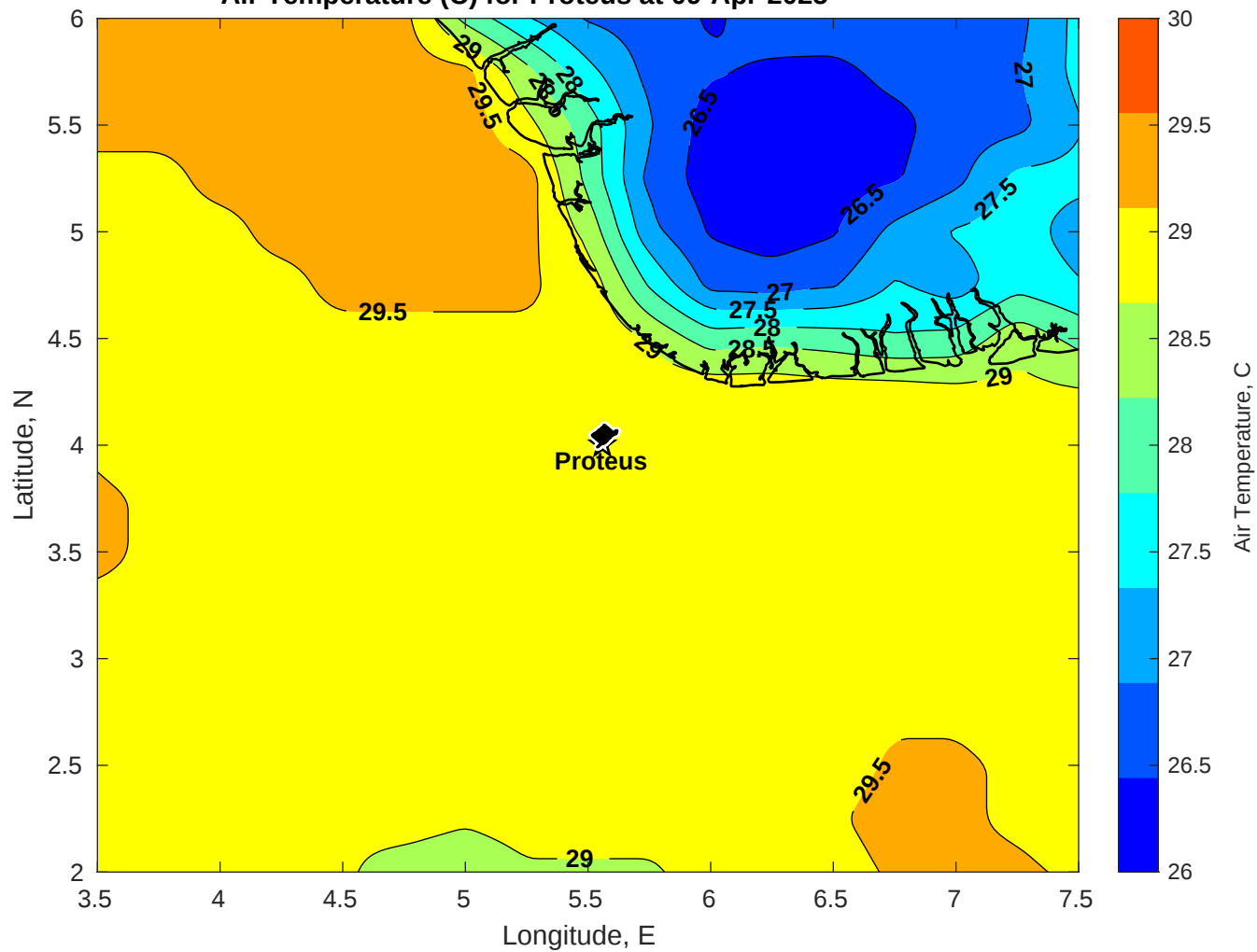
Air Temperature (C) for Proteus at 09-Apr-2025
