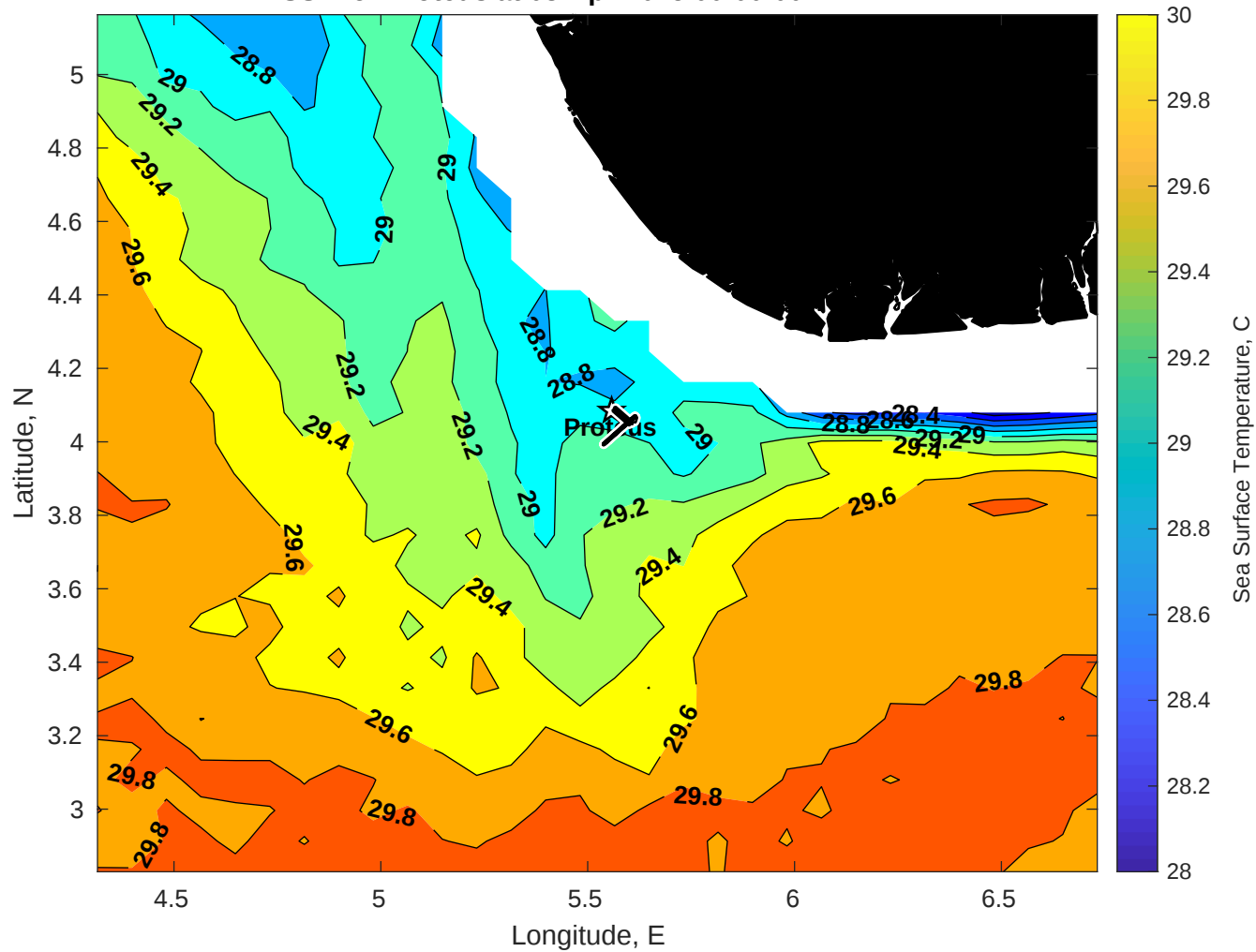
SST for Proteus at 08-Apr-2025 00:00:00
