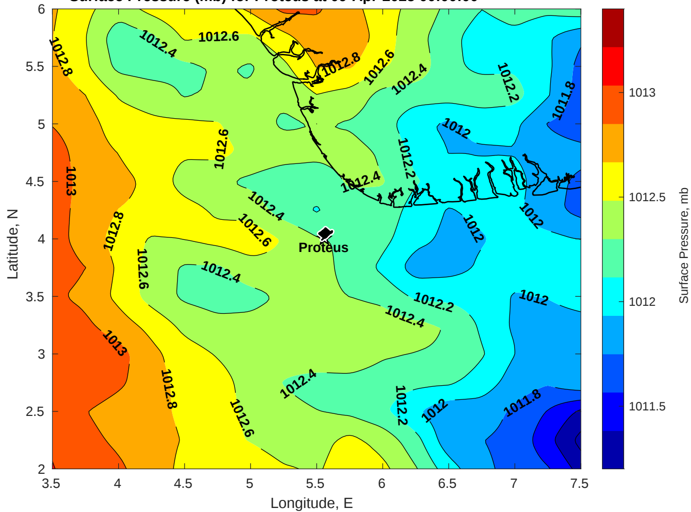
Surface Pressure (mb) for Proteus at 09-Apr-2025 00:00:00
