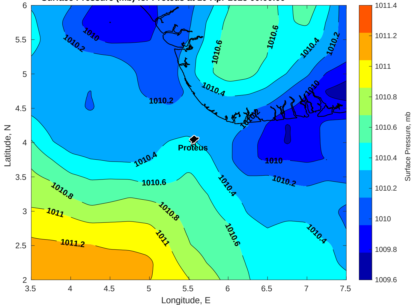
Surface Pressure (mb) for Proteus at 10-Apr-2025 00:00:00
