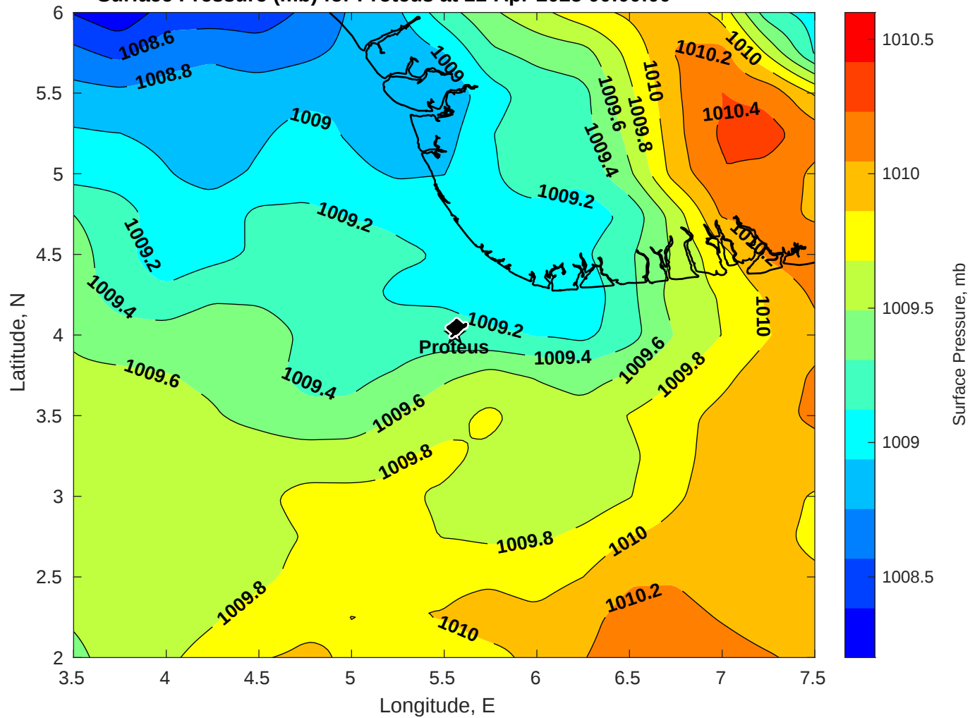
Surface Pressure (mb) for Proteus at 11-Apr-2025 00:00:00
