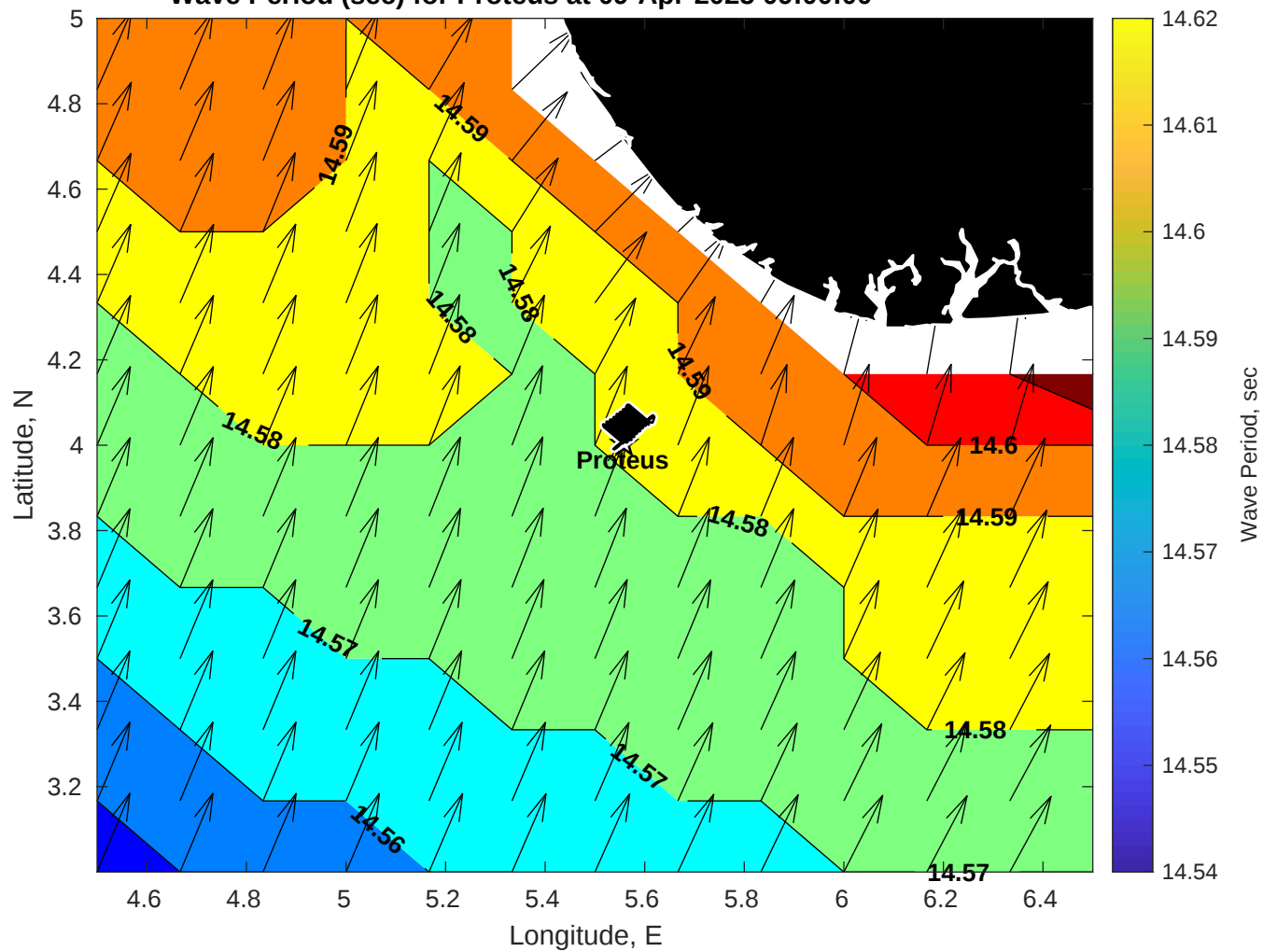
Wave Period (sec) for Proteus at 09-Apr-2025 09:00:00
