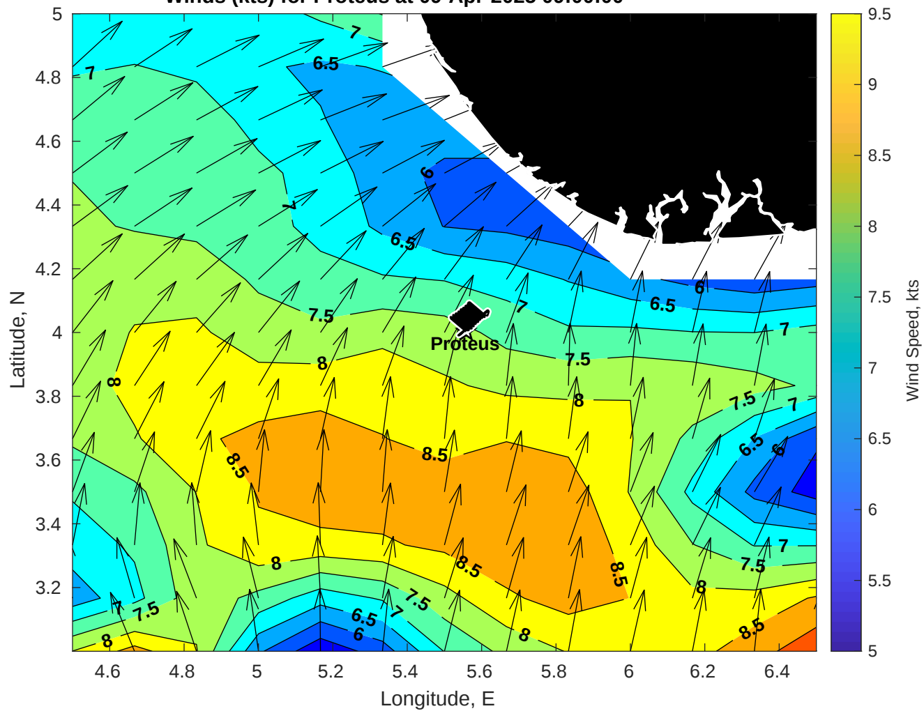
Winds (kts) for Proteus at 09-Apr-2025 09:00:00
