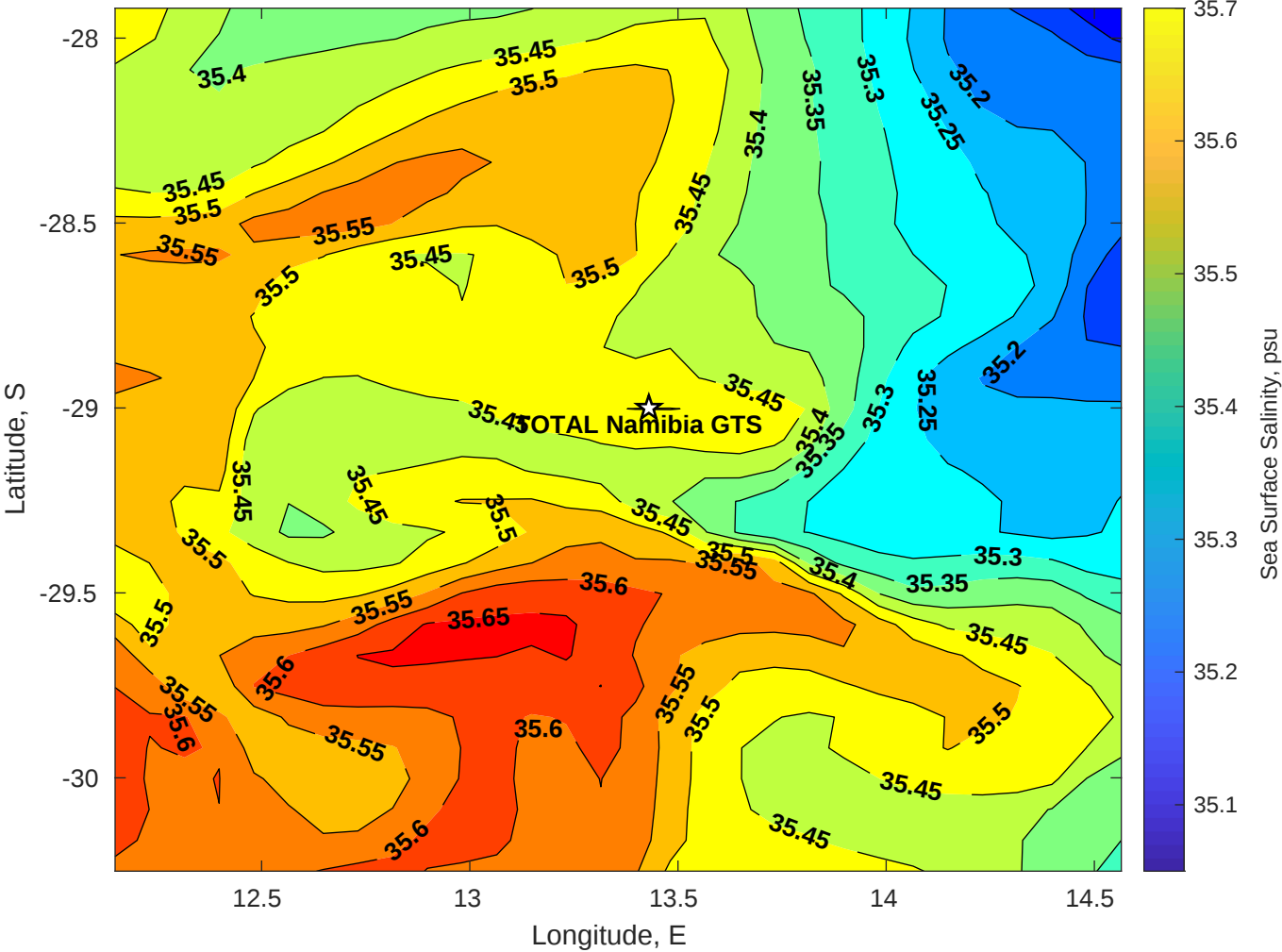
Surface Salinity for TOTAL Namibia GTS at 08-Apr-2025 00:00:00
