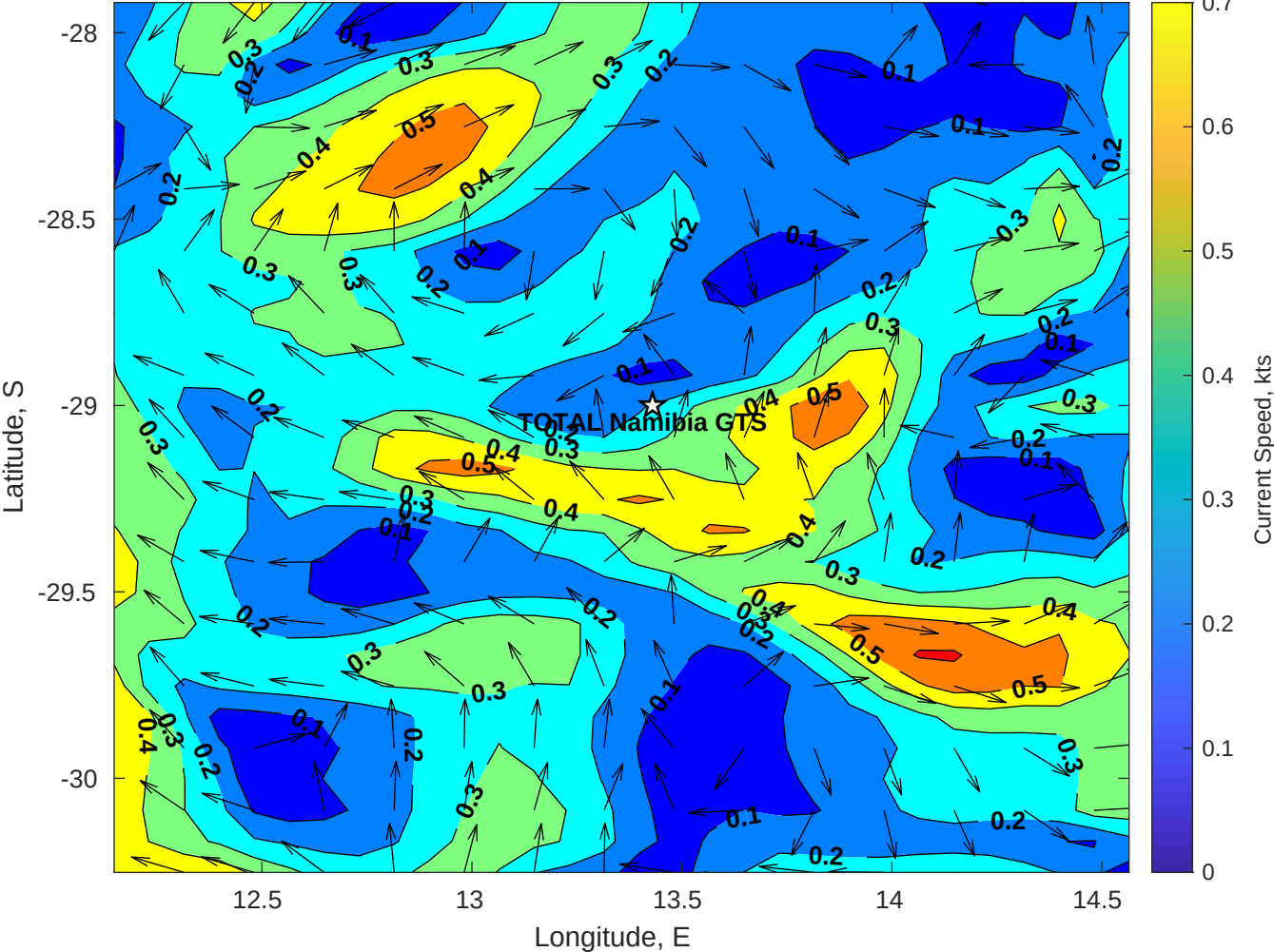
Surface Currents for TOTAL Namibia GTS at 08-Apr-2025 00:00:00
