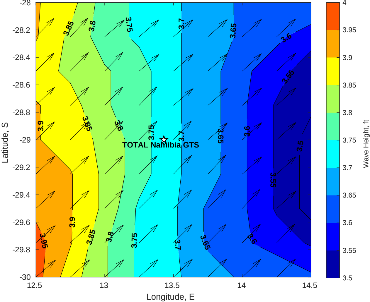
Wave Height (ft) for TOTAL Namibia GTS at 09-Apr-2025 09:00:00
