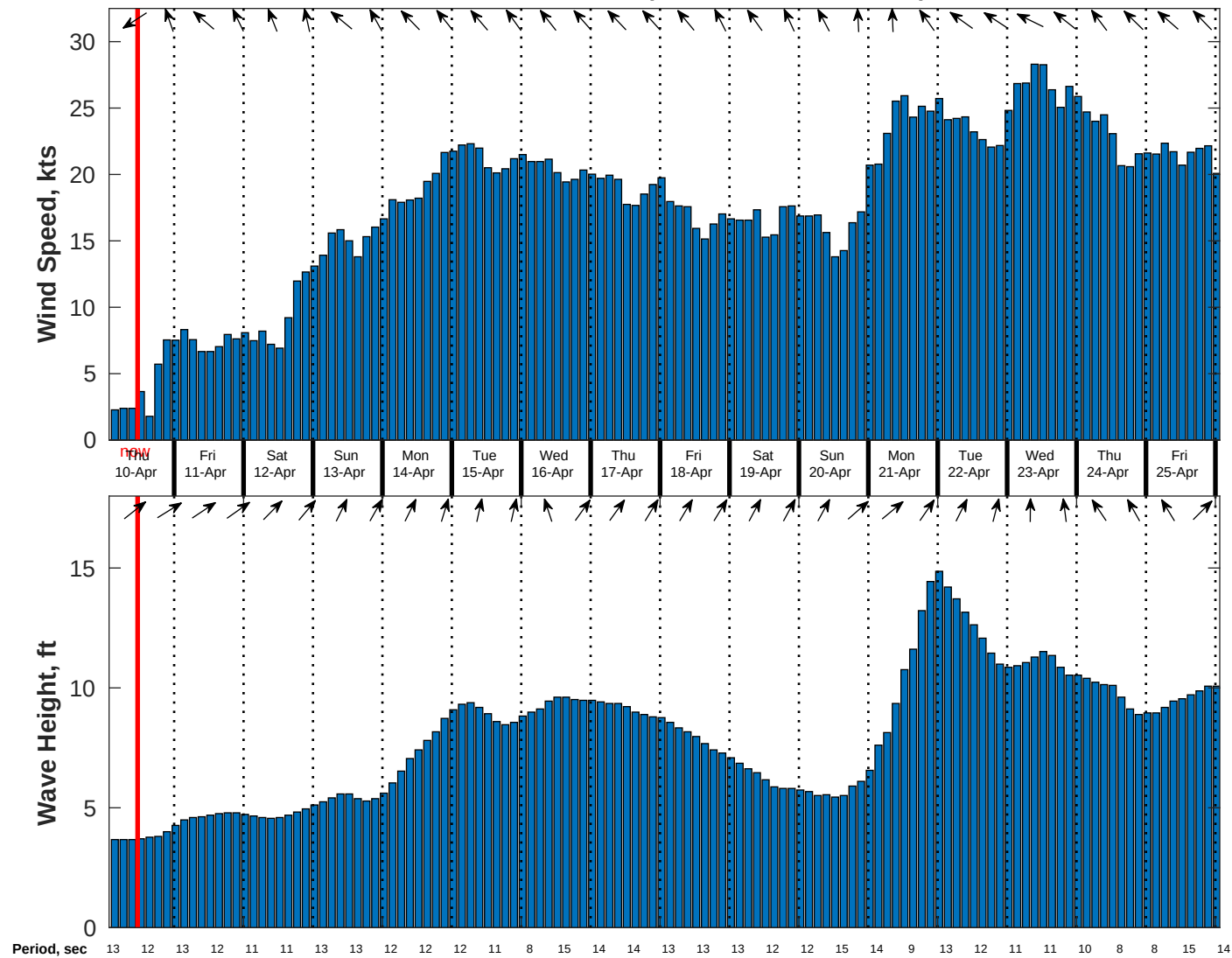
Wind & Wave Forecast for TOTAL Namibia GTS from 09-Apr-2025 02:00:00 to 25-Apr-2025 02:00:00
