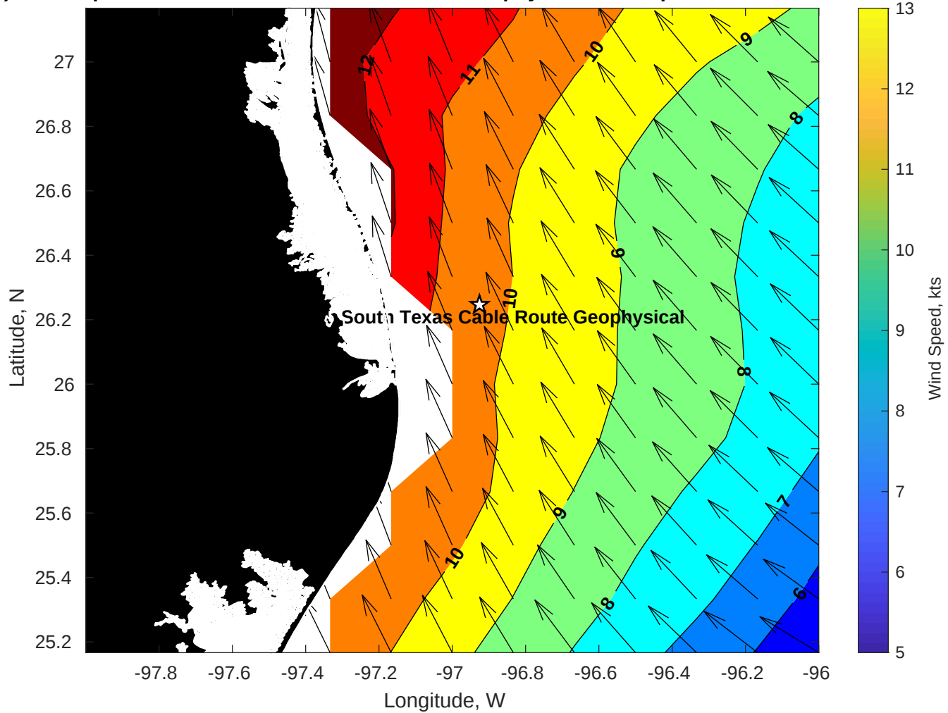
Winds (kts) for Tampnet P2378 South Texas Cable Route Geophysical at 09-Apr-2025 09:00:00
