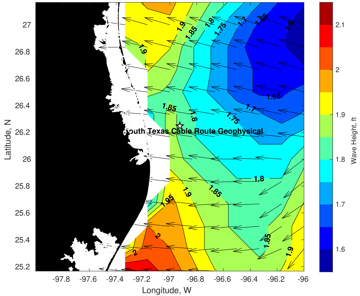
Wave Height (ft) for Tampnet P2378 South Texas Cable Route Geophysical at 09-Apr-2025 09:00:00
