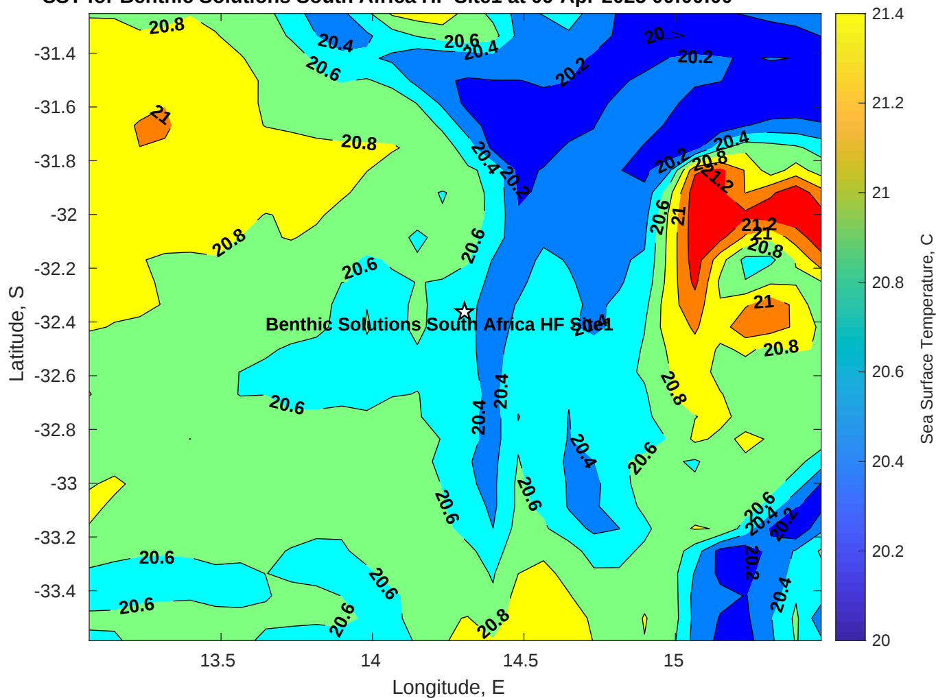
SST for Benthic Solutions South Africa HF Site1 at 09-Apr-2025 00:00:00
