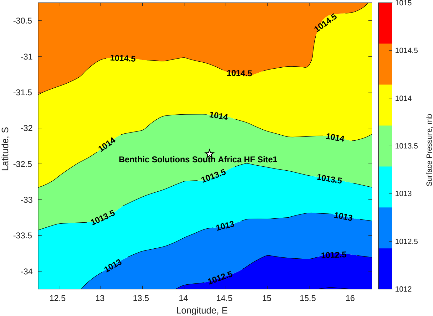
Surface Pressure (mb) for Benthic Solutions South Africa HF Site1 at 12-Apr-2025 00:00:00
