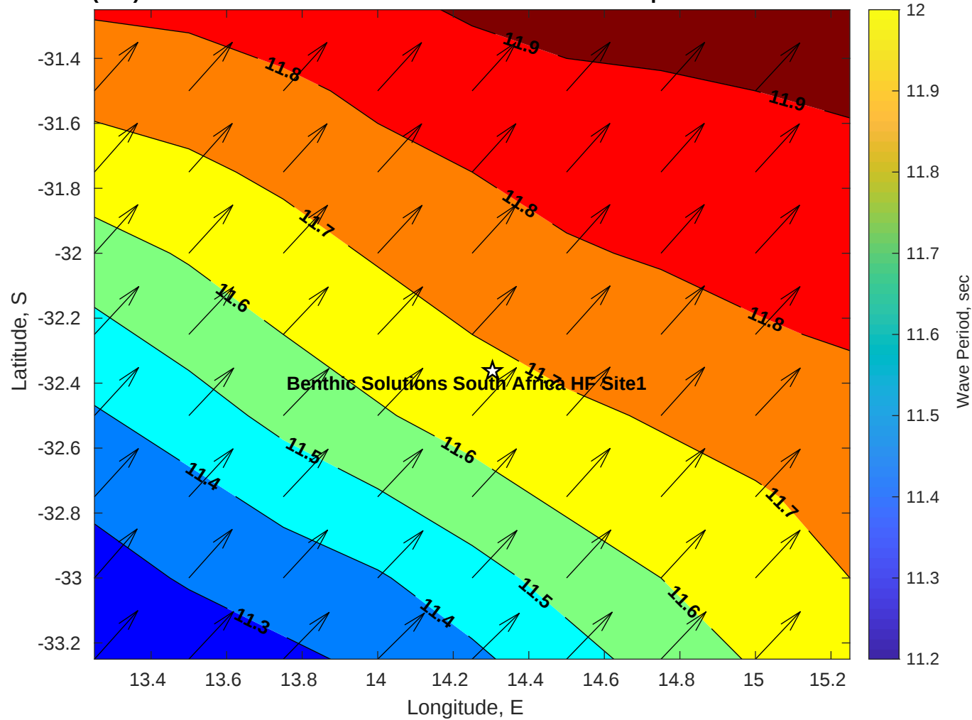
Wave Period (sec) for Benthic Solutions South Africa HF Site1 at 10-Apr-2025 09:00:00
