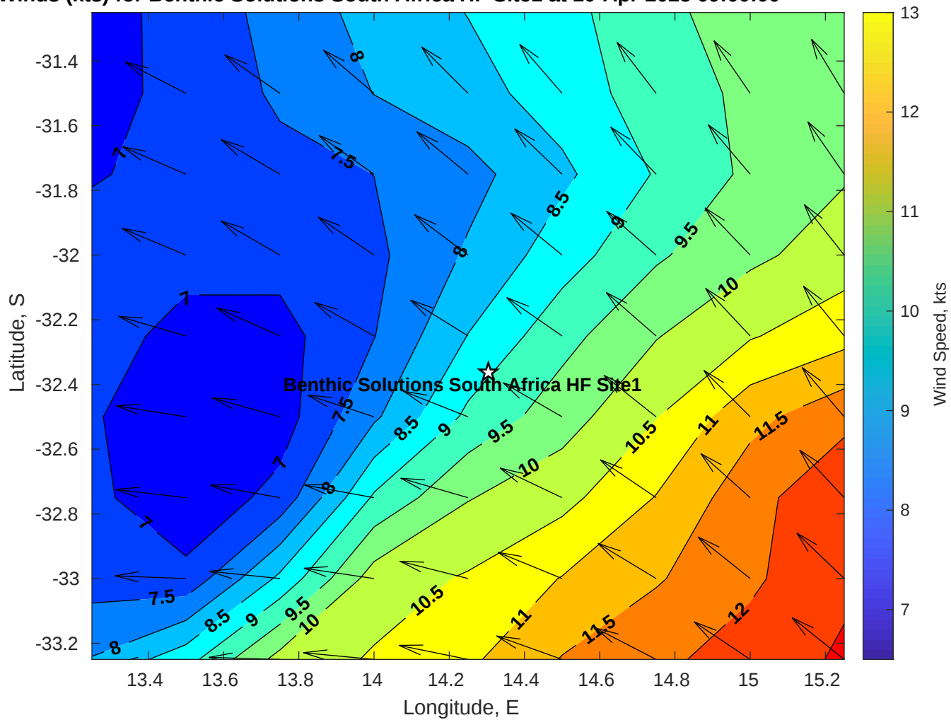
Winds (kts) for Benthic Solutions South Africa HF Site1 at 10-Apr-2025 09:00:00
