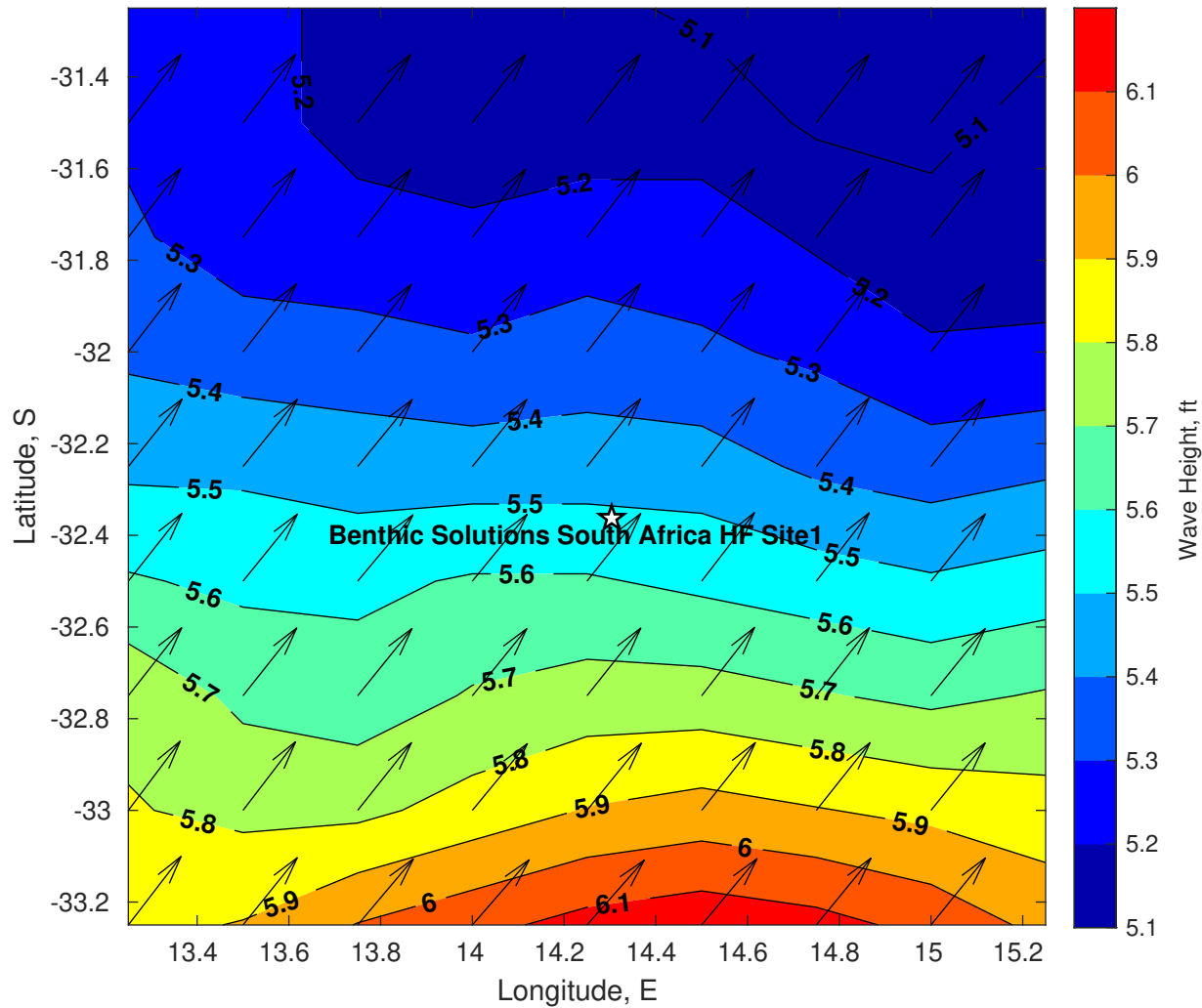
Wave Height (ft) for Benthic Solutions South Africa HF Site1 at 10-Apr-2025 09:00:00
