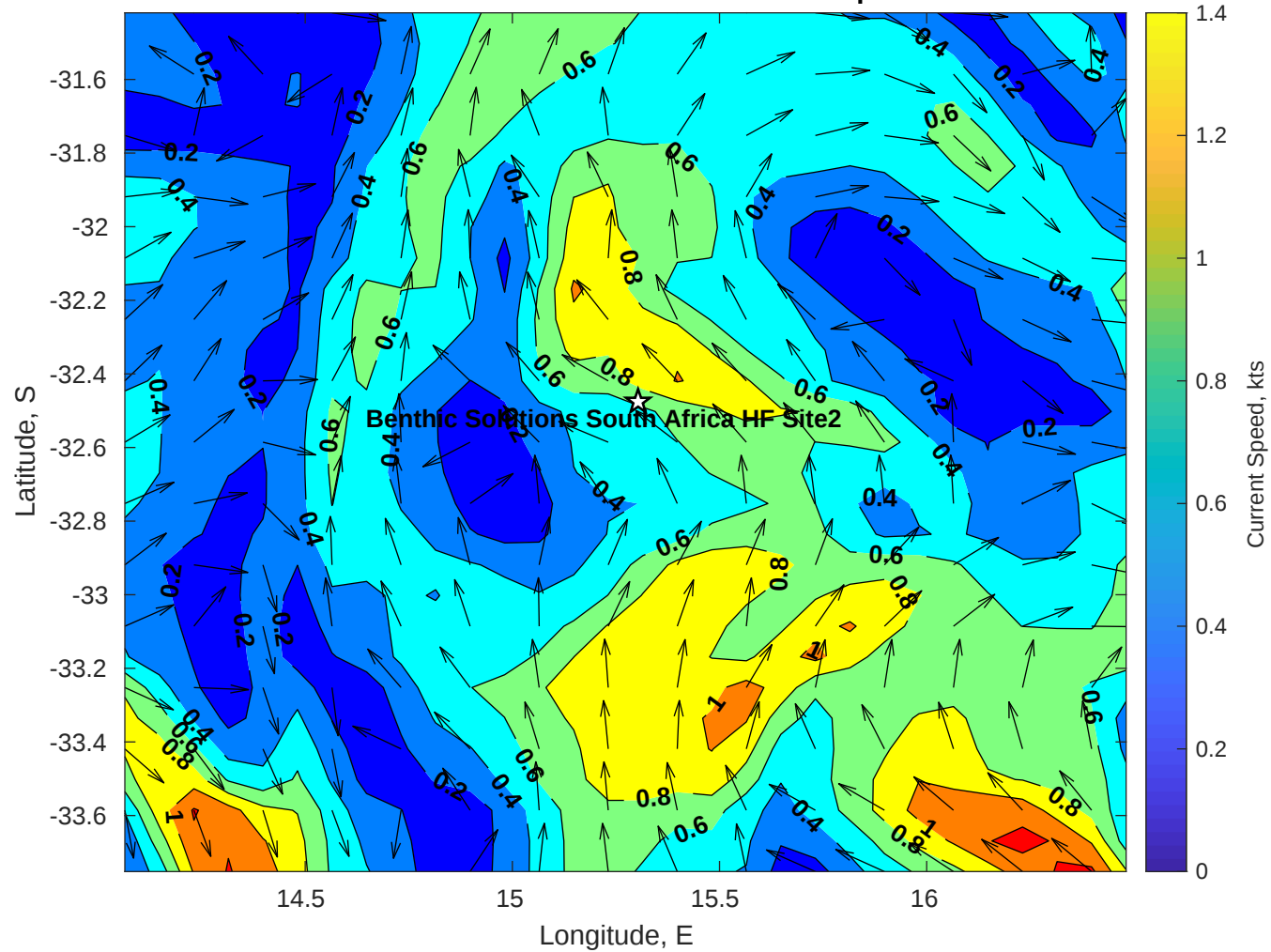
Surface Currents for Benthic Solutions South Africa HF Site2 at 09-Apr-2025 00:00:00
