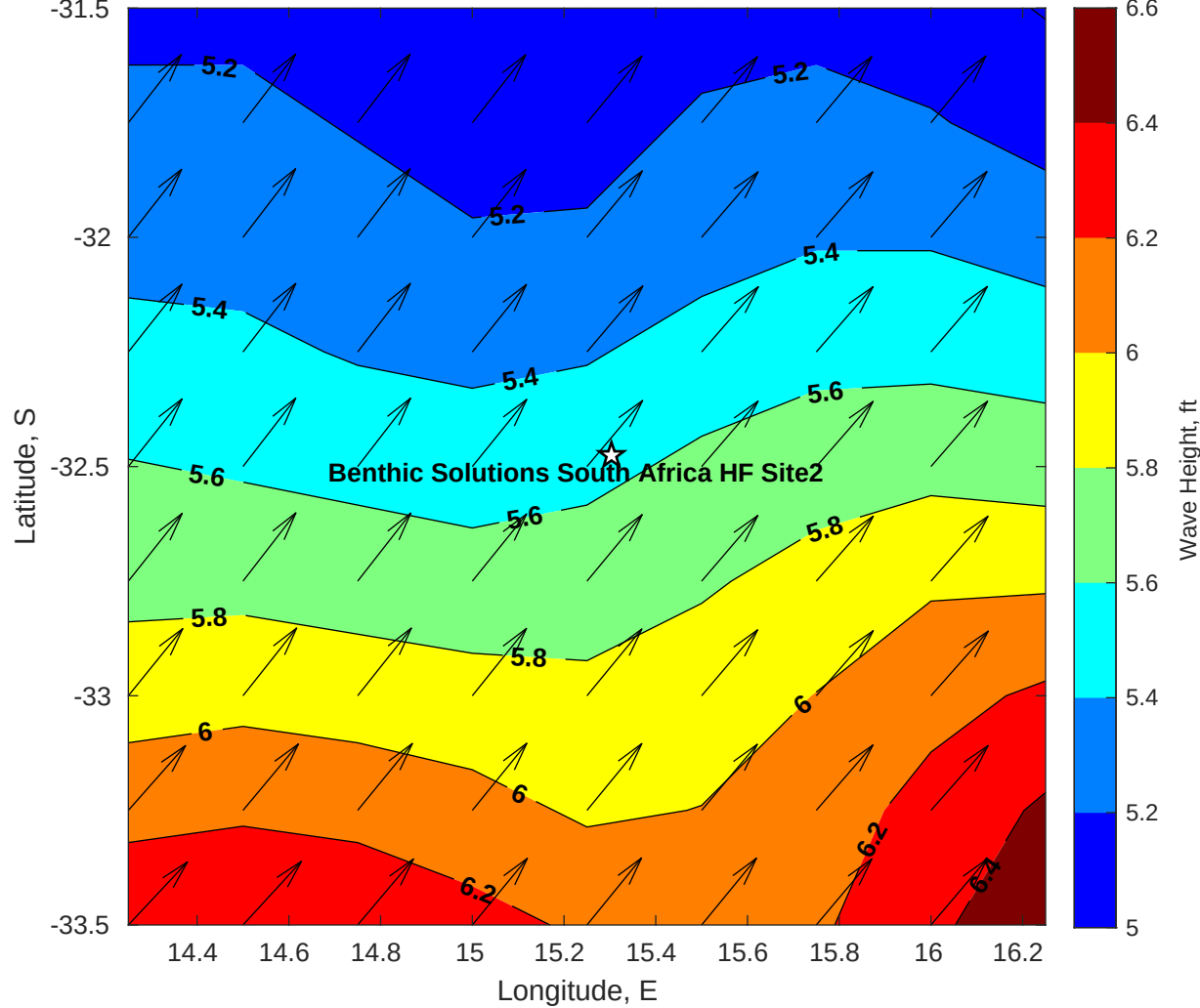
Wave Height (ft) for Benthic Solutions South Africa HF Site2 at 10-Apr-2025 09:00:00
