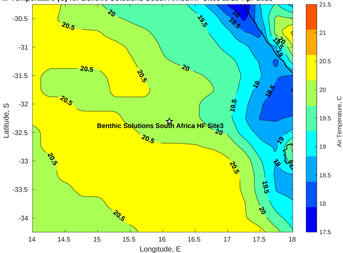
Air Temperature (C) for Benthic Solutions South Africa HF Site3 at 10-Apr-2025
