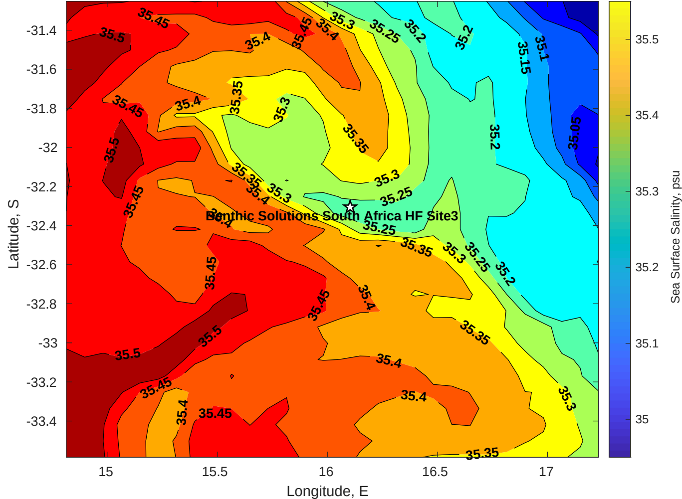
Surface Salinity for Benthic Solutions South Africa HF Site3 at 09-Apr-2025 00:00:00
