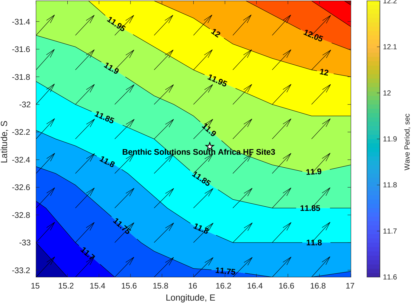
Wave Period (sec) for Benthic Solutions South Africa HF Site3 at 10-Apr-2025 09:00:00
