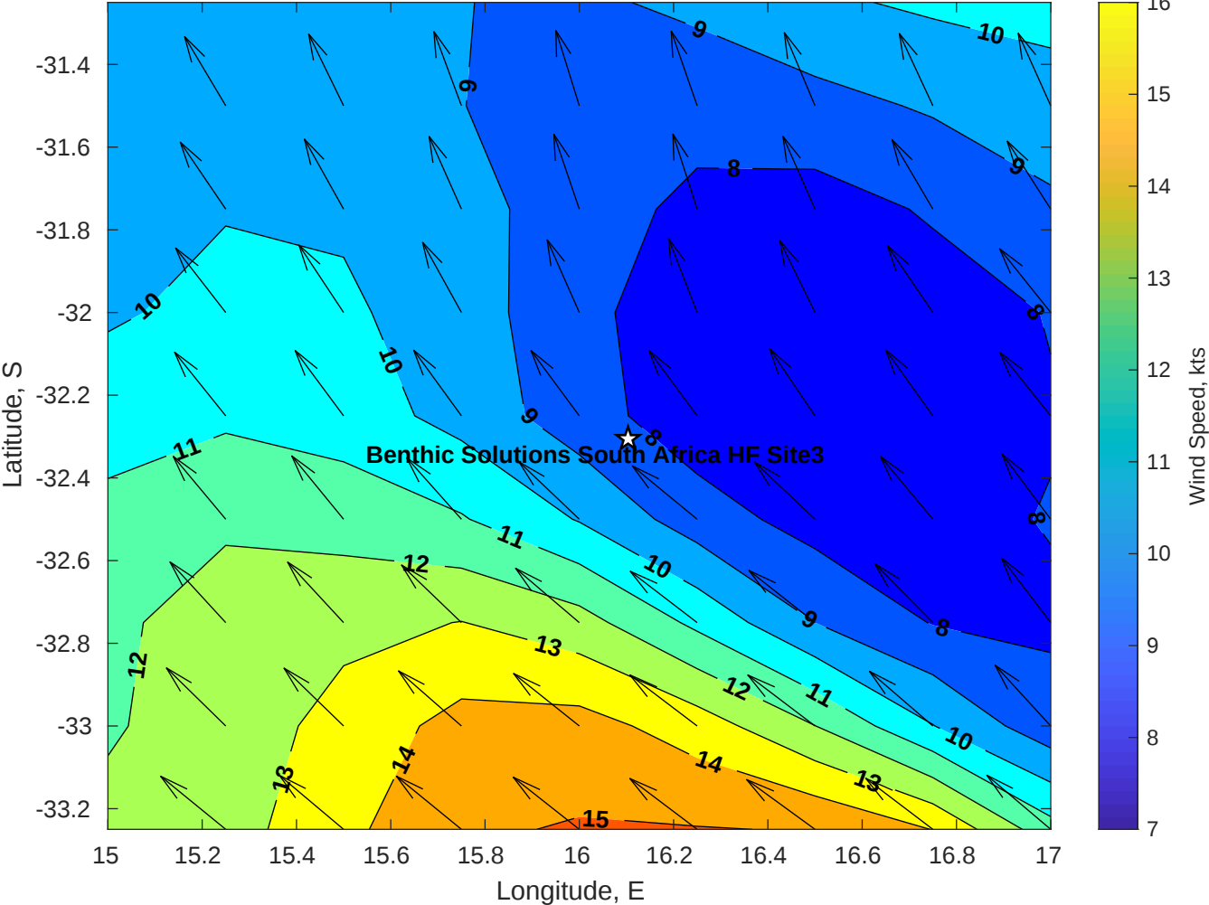
Winds (kts) for Benthic Solutions South Africa HF Site3 at 10-Apr-2025 09:00:00
