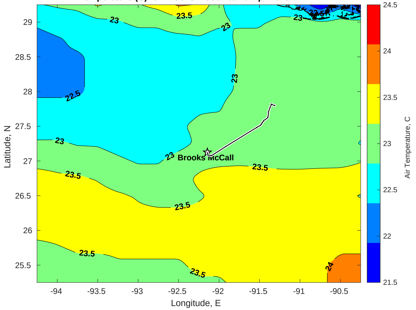
Air Temperature (C) for Brooks McCall at 10-Apr-2025
