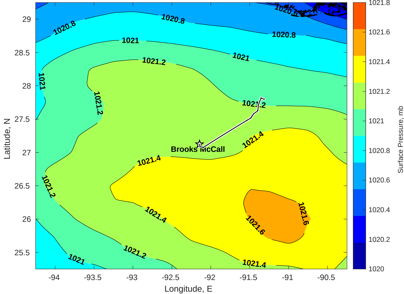
Surface Pressure (mb) for Brooks McCall at 11-Apr-2025 00:00:00
