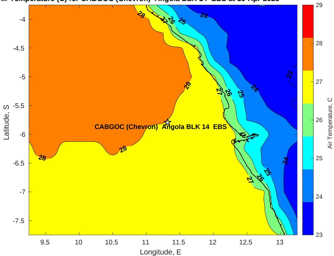
Air Temperature (C) for CABGOC (Chevron) Angola BLK 14 EBS at 10-Apr-2025
