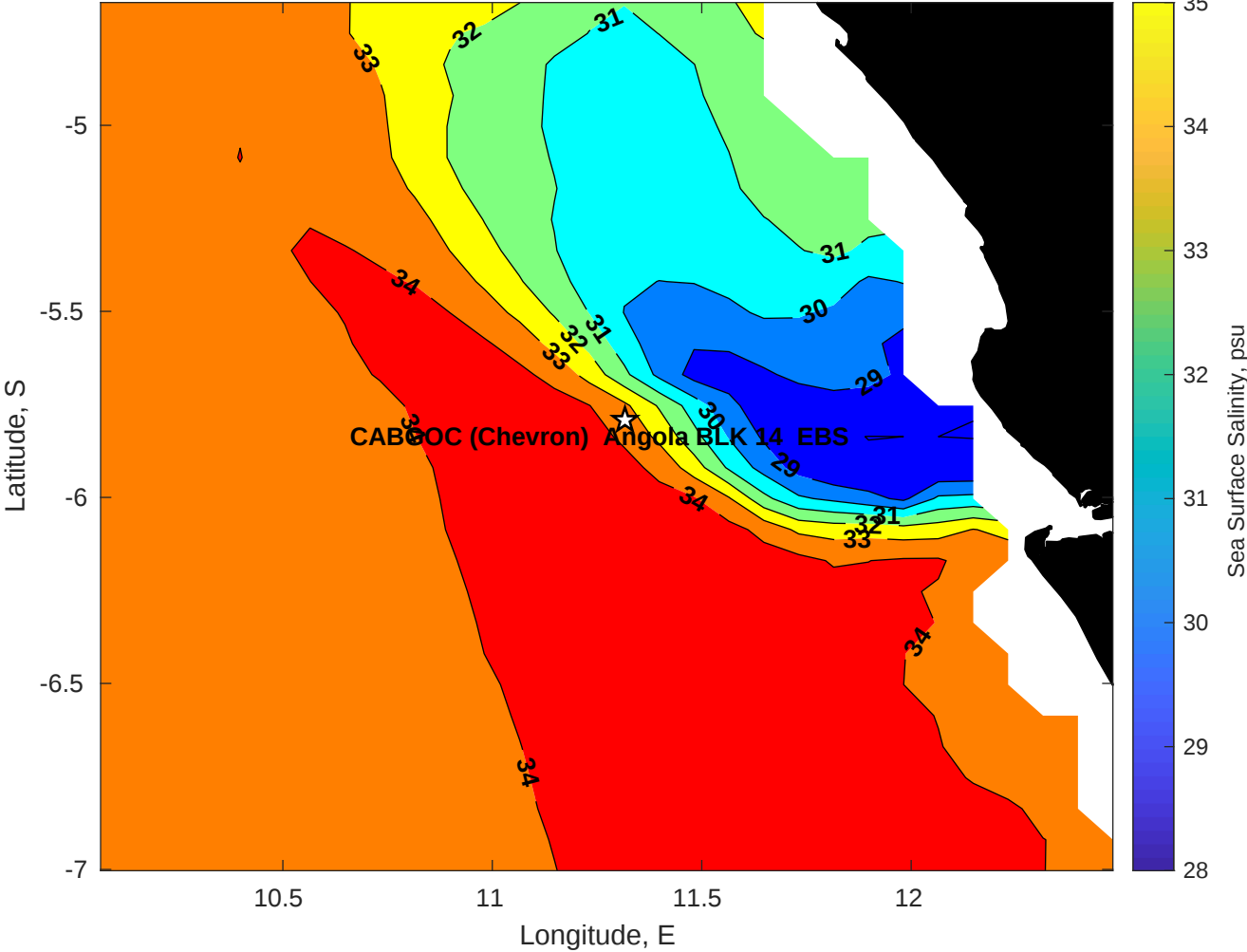
Surface Salinity for CABGOC (Chevron) Angola BLK 14 EBS at 09-Apr-2025 00:00:00
