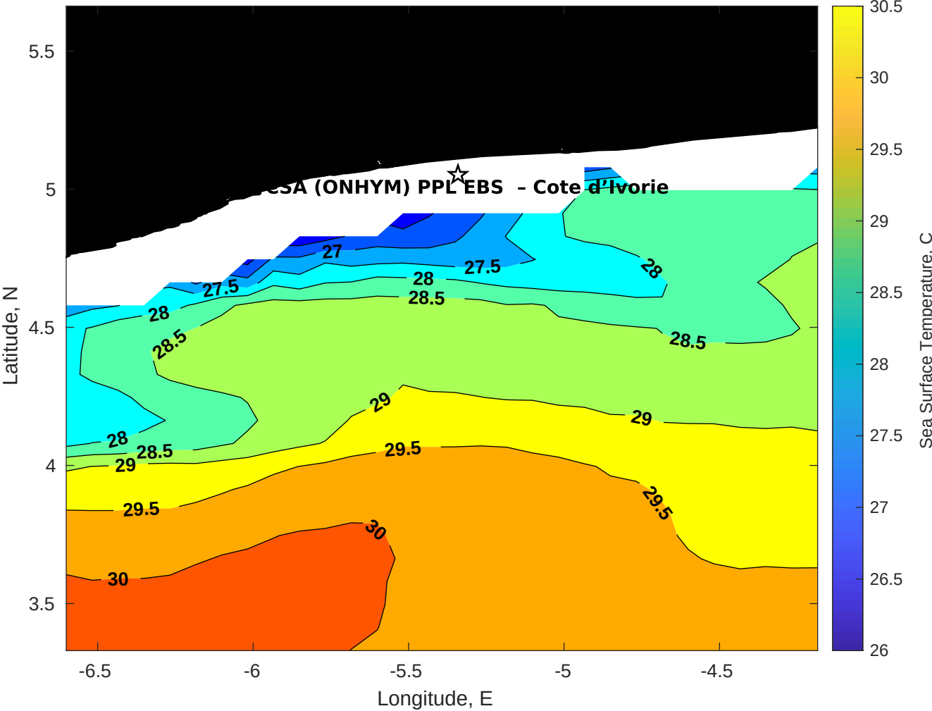
SST for CSA (ONHYM) PPL EBS - Cote d'Ivoire at 09-Apr-2025 00:00:00
