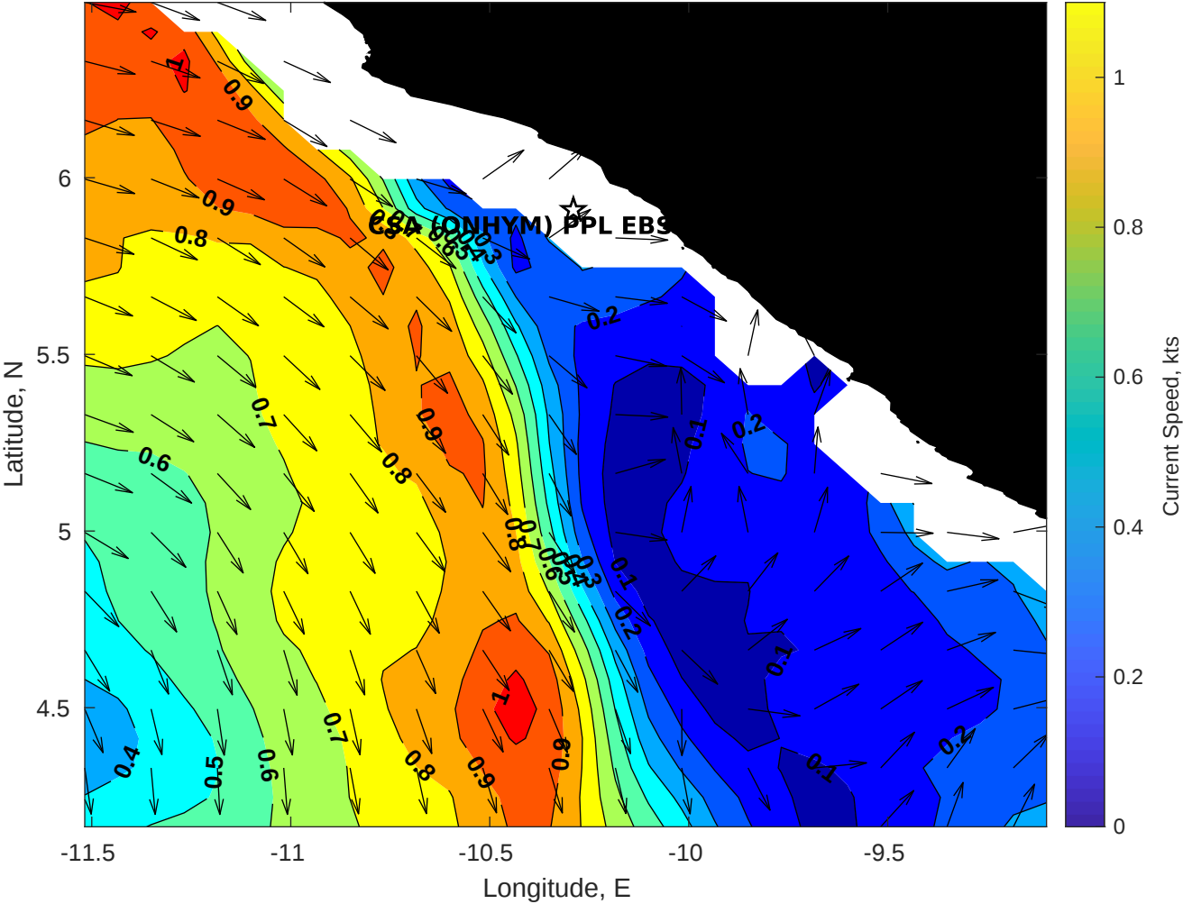
Surface Currents for CSA (ONHYM) PPL EBS - Liberia at 09-Apr-2025 00:00:00
