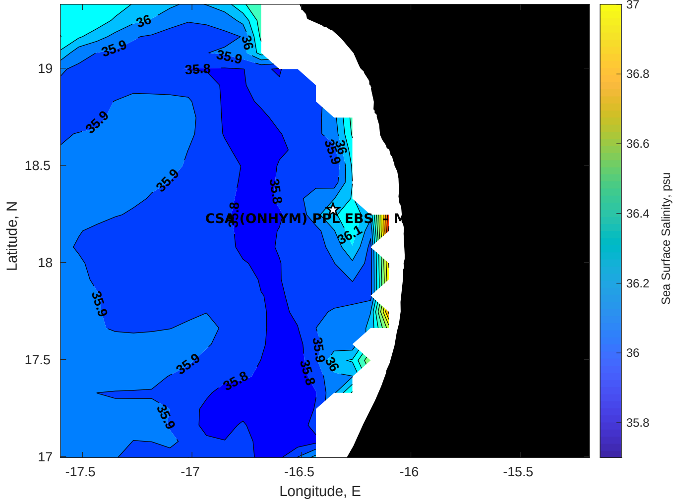
Surface Salinity for CSA (ONHYM) PPL EBS - Mauritania at 09-Apr-2025 00:00:00
