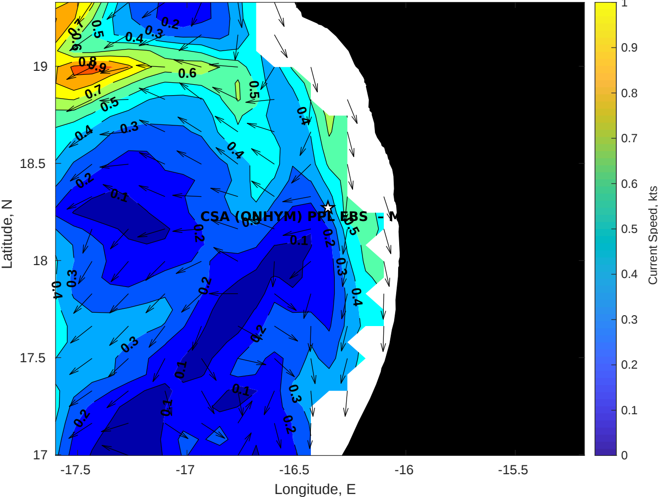
Surface Currents for CSA (ONHYM) PPL EBS - Mauritania at 09-Apr-2025 00:00:00
