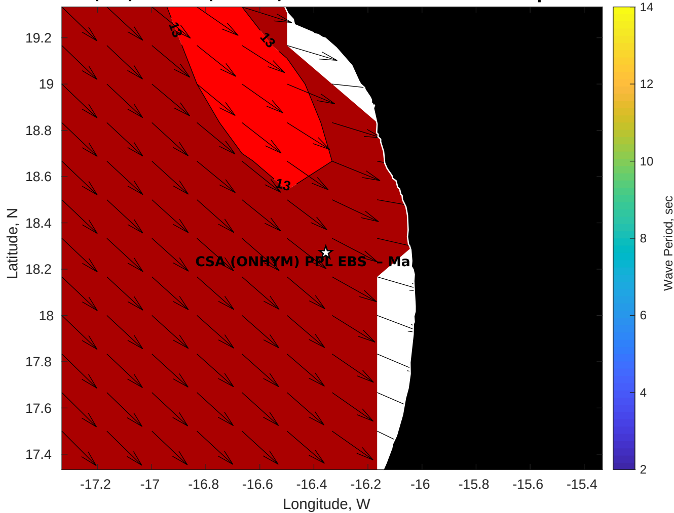
Wave Period (sec) for CSA (ONHYM) PPL EBS - Mauritania at 10-Apr-2025 09:00:00
