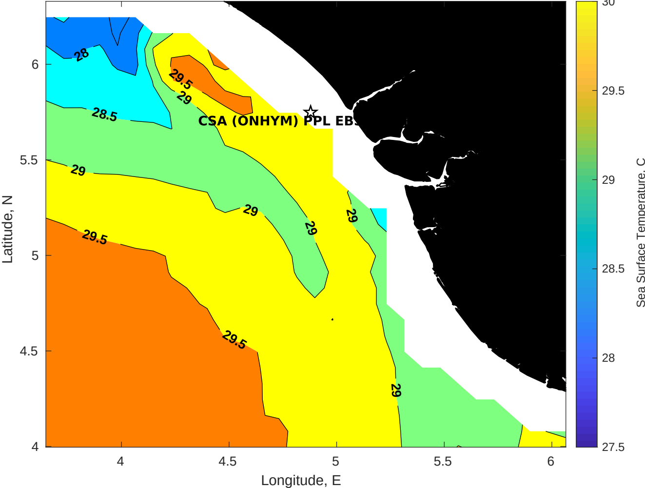
SST for CSA (ONHYM) PPL EBS - Nigeria at 09-Apr-2025 00:00:00
