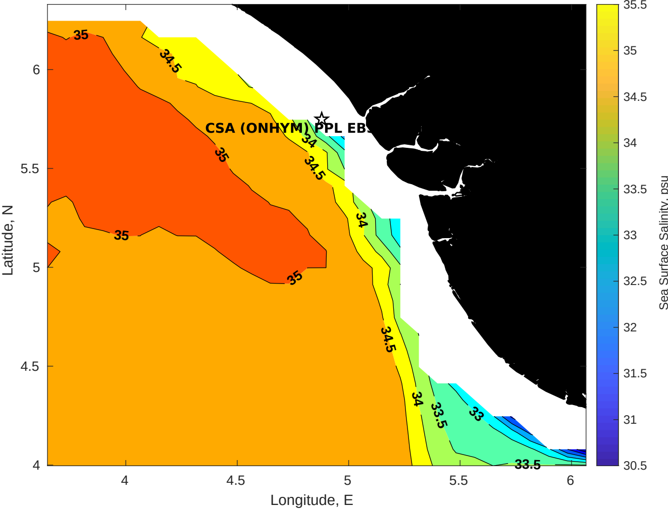
Surface Salinity for CSA (ONHYM) PPL EBS - Nigeria at 09-Apr-2025 00:00:00
