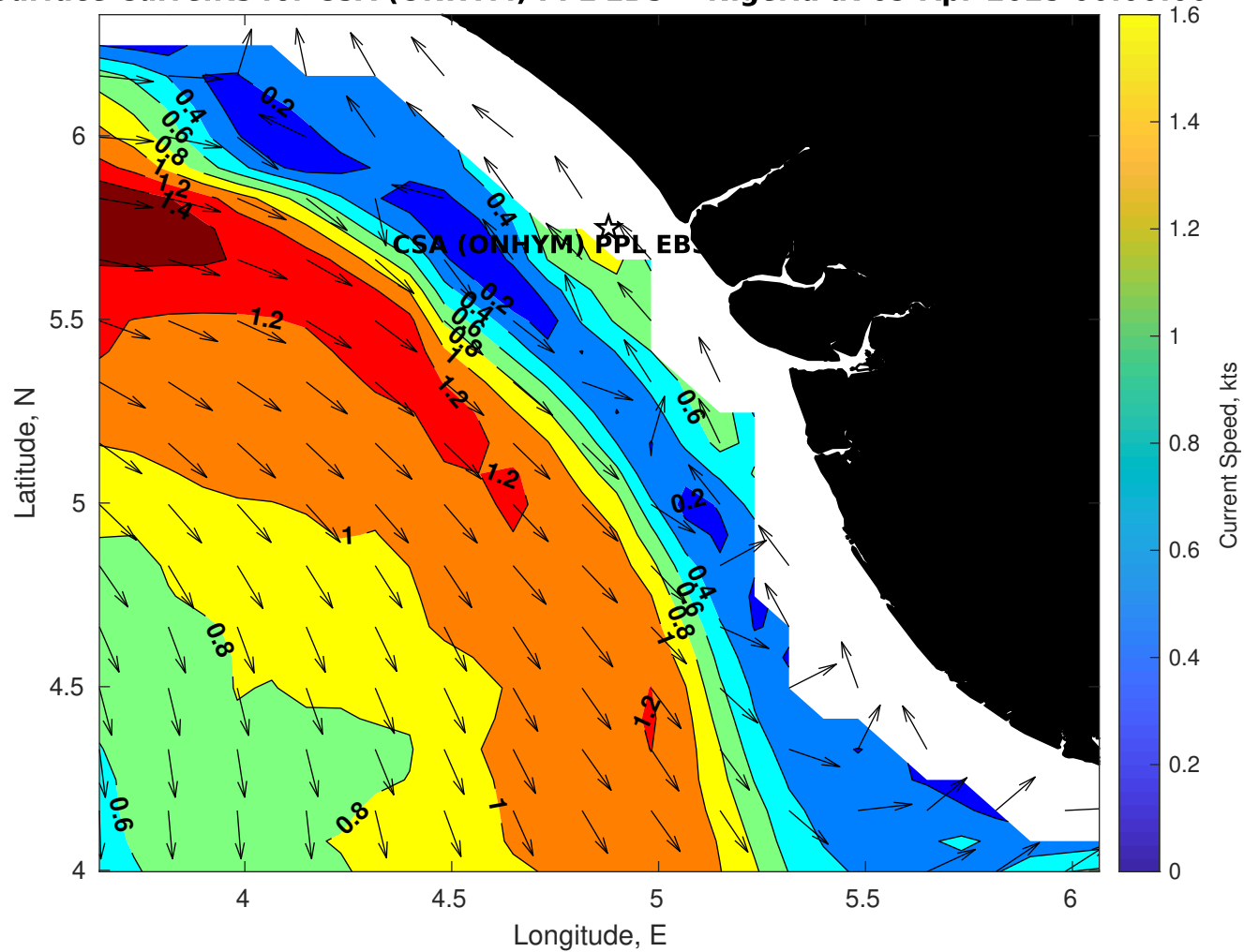
Surface Currents for CSA (ONHYM) PPL EBS - Nigeria at 09-Apr-2025 00:00:00
