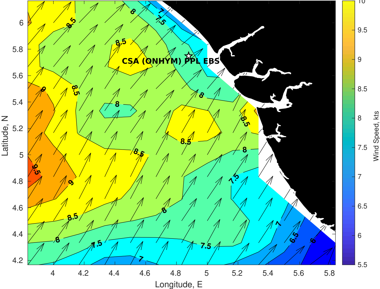
Winds (kts) for CSA (ONHYM) PPL EBS - Nigeria at 10-Apr-2025 09:00:00
