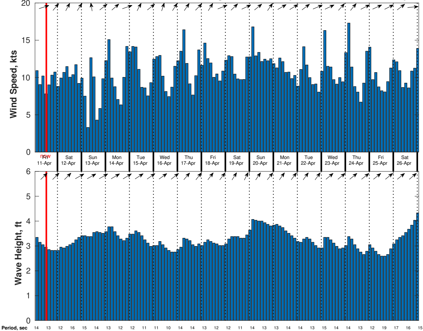
Wind & Wave Forecast for CSA (ONHYM) PPL EBS - Nigeria from 10-Apr-2025 02:00:00 to 26-Apr-2025 02:00:00
