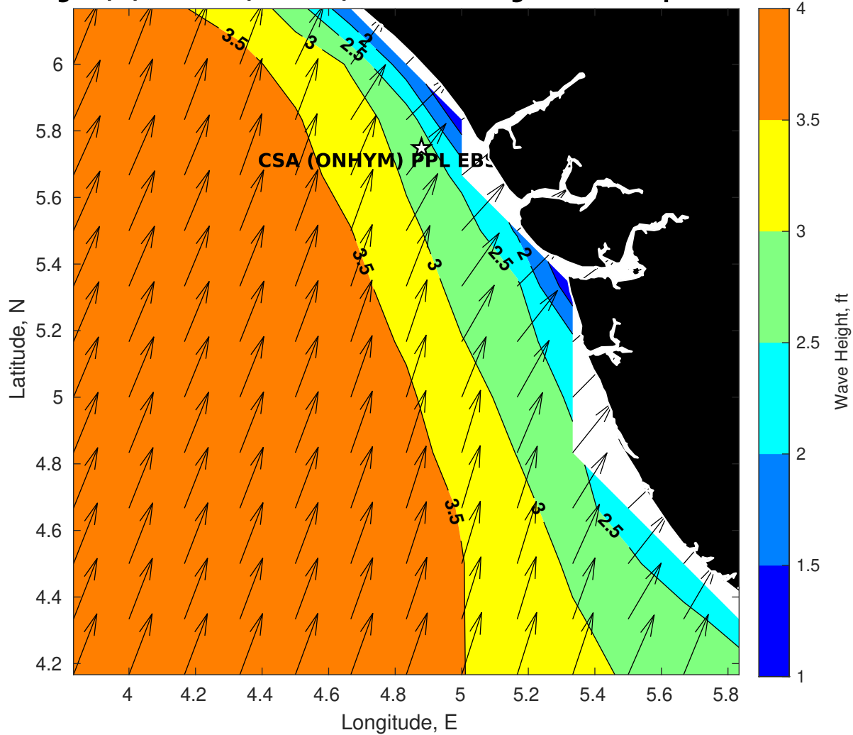
Wave Height (ft) for CSA (ONHYM) PPL EBS - Nigeria at 10-Apr-2025 09:00:00
