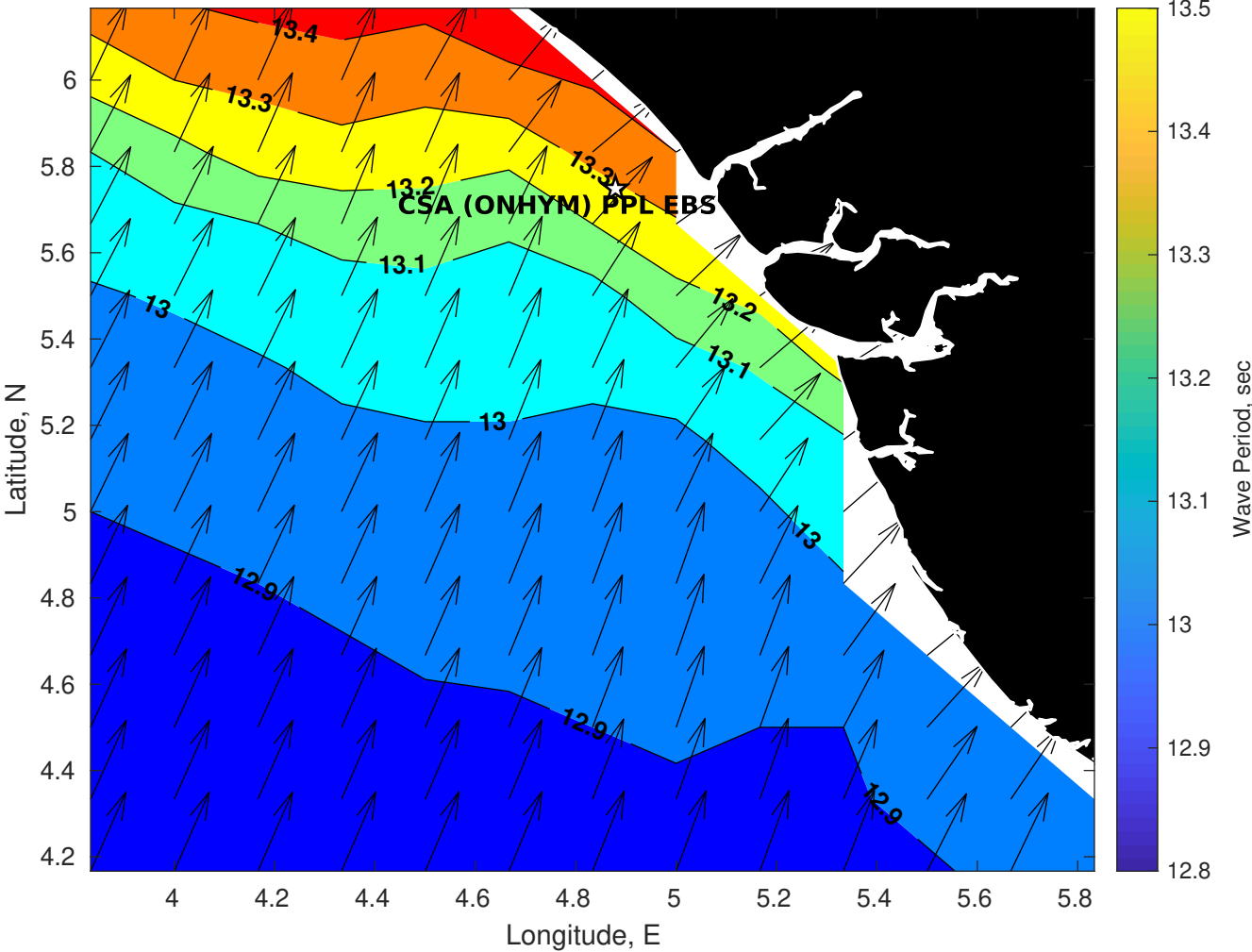
Wave Period (sec) for CSA (ONHYM) PPL EBS - Nigeria at 10-Apr-2025 09:00:00
