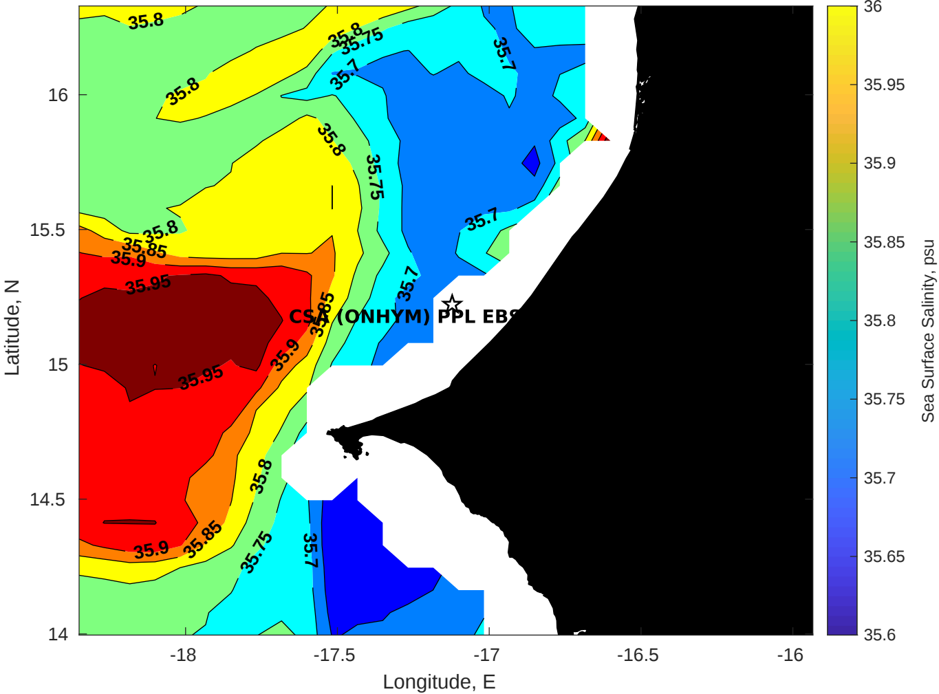
Surface Salinity for CSA (ONHYM) PPL EBS - Senegal at 09-Apr-2025 00:00:00
