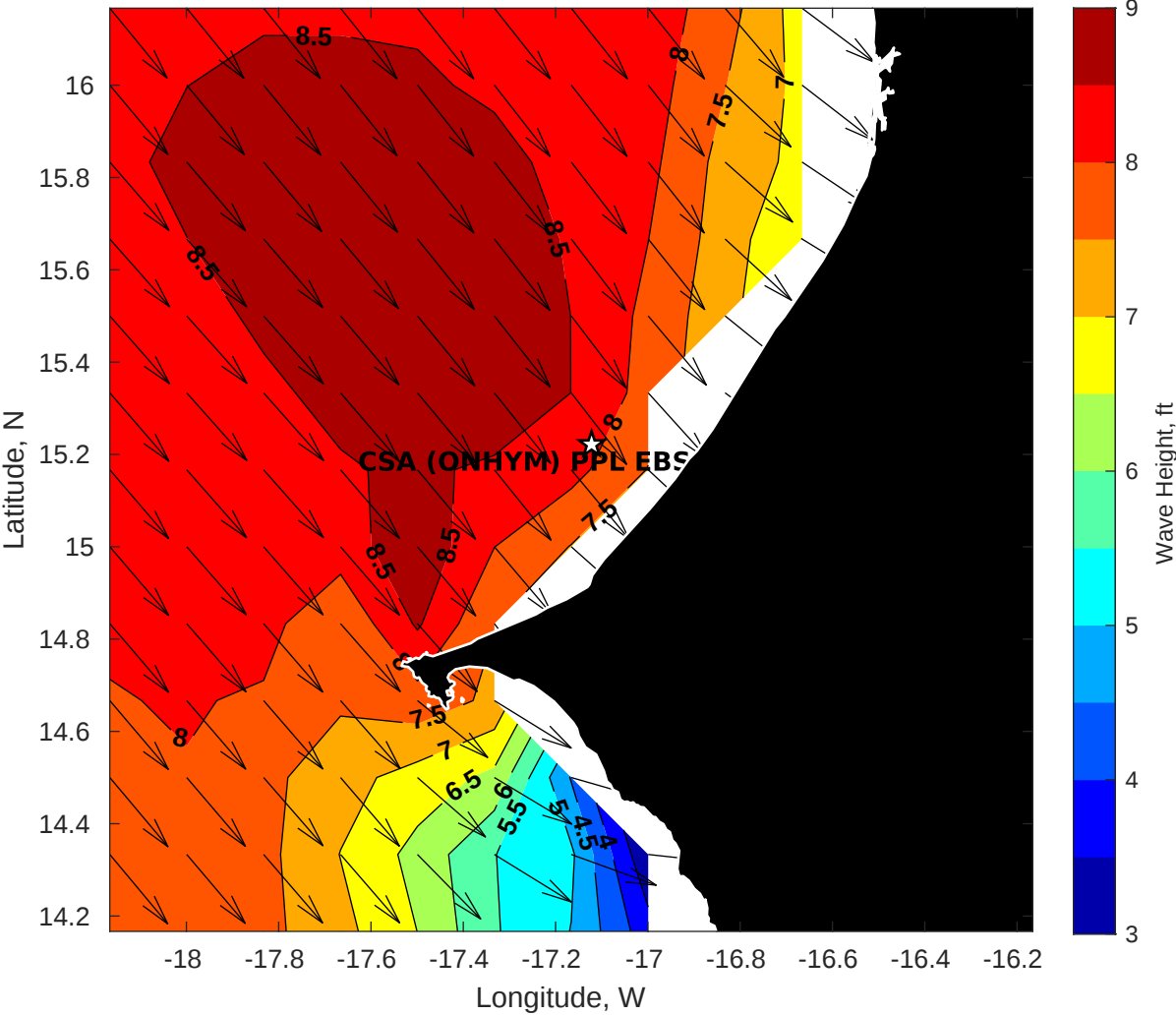
Wave Height (ft) for CSA (ONHYM) PPL EBS - Senegal at 10-Apr-2025 09:00:00
