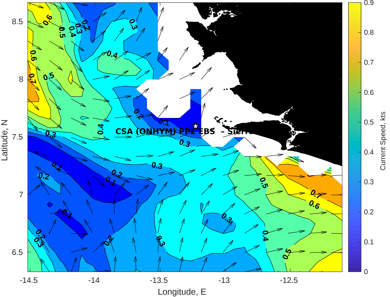
Surface Currents for CSA (ONHYM) PPL EBS - Sierra Leone at 09-Apr-2025 00:00:00
