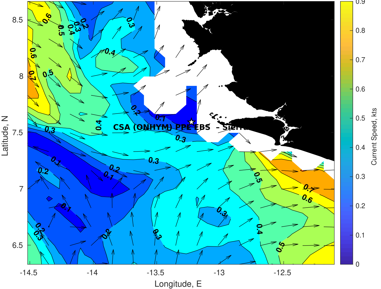
Surface Currents for CSA (ONHYM) PPL EBS - Sierra Leone at 09-Apr-2025 00:00:00
