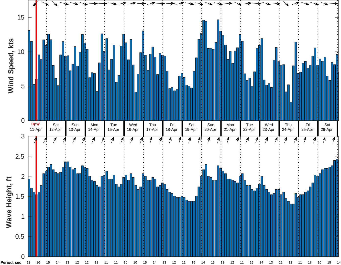
Wind & Wave Forecast for CSA (ONHYM) PPL EBS - Sierra Leone from 10-Apr-2025 01:00:00 to 26-Apr-2025 01:00:00
