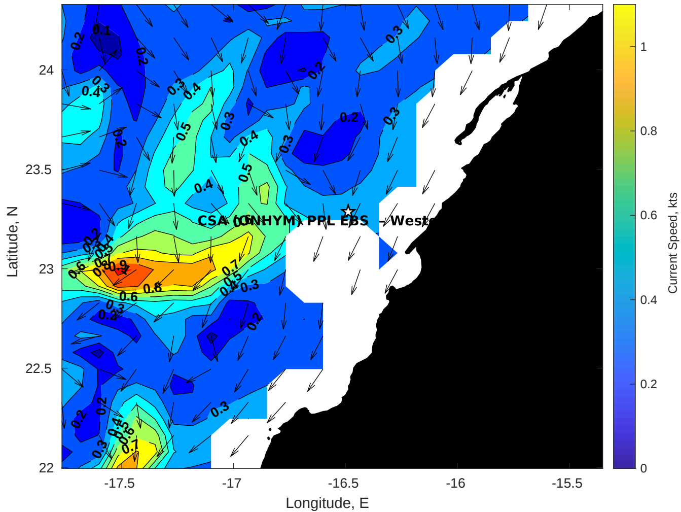
Surface Currents for CSA (ONHYM) PPL EBS - Western Sahara at 09-Apr-2025 00:00:00
