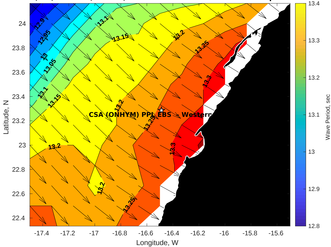
Wave Period (sec) for CSA (ONHYM) PPL EBS - Western Sahara at 10-Apr-2025 09:00:00
