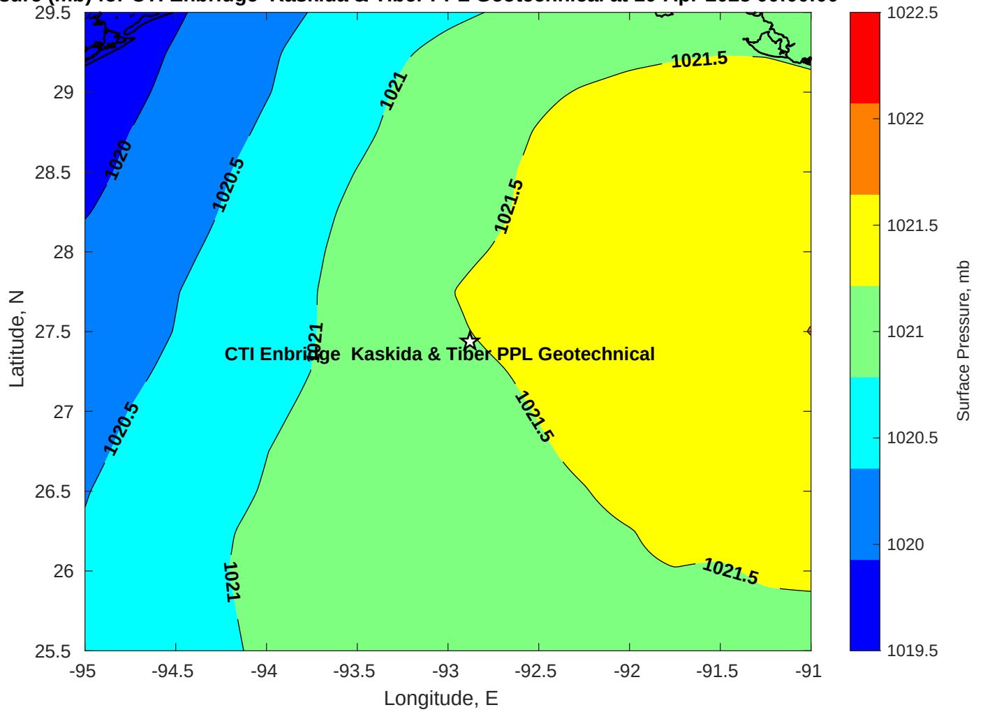
Surface Pressure (mb) for CTI Enbridge Kaskida & Tiber PPL Geotechnical at 10-Apr-2025 00:00:00
