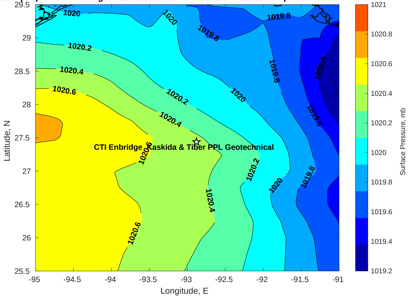
Surface Pressure (mb) for CTI Enbridge Kaskida & Tiber PPL Geotechnical at 12-Apr-2025 00:00:00
